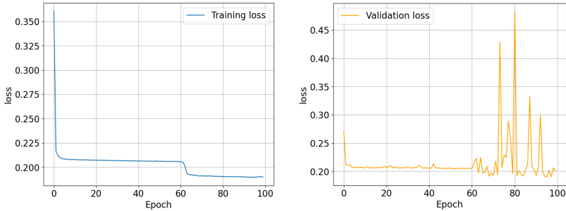
Fig. 5. Training Vs validation loss
